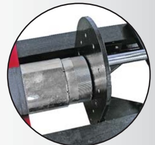
Faster & Safer Industrial Fitting Insertion
